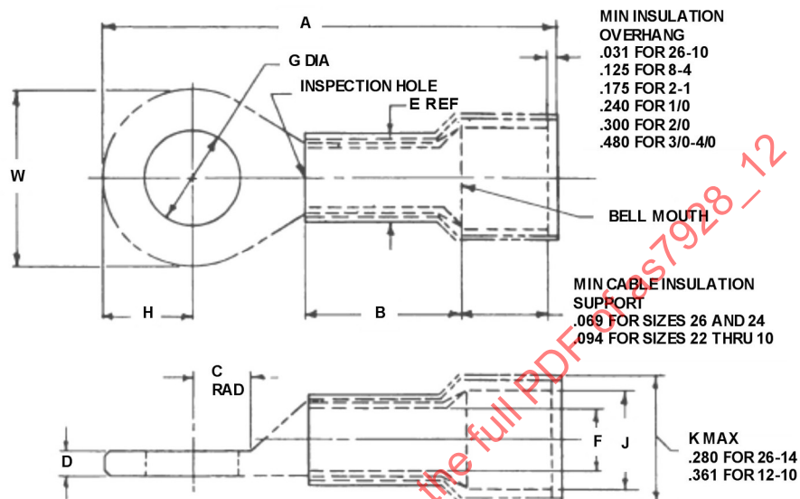
FIGURE 1 - TERMINAL CONSTRUCTION
