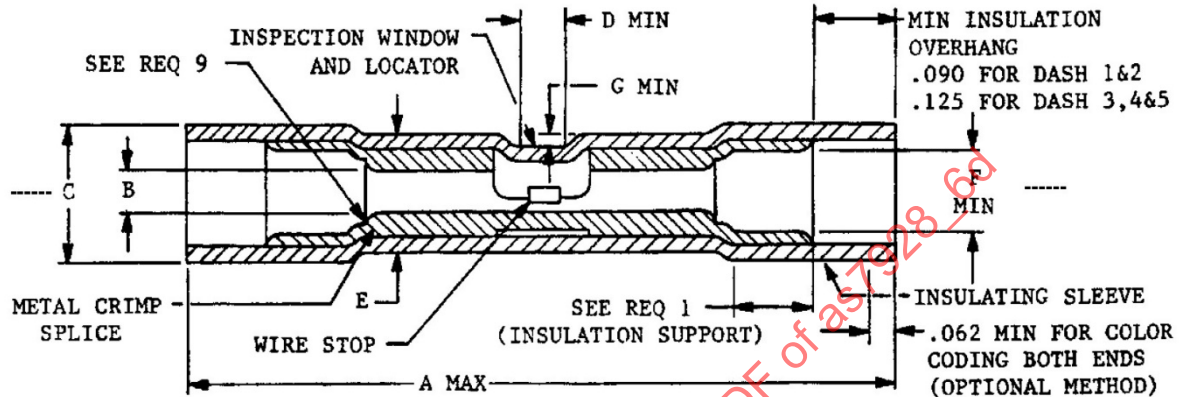
FIGURE 1 - AS7928/6 SPLICE
