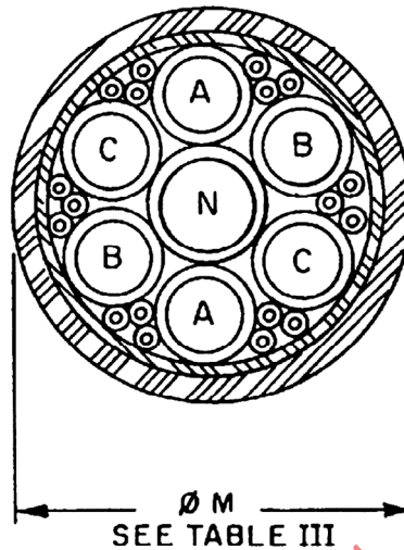
TYPE II, STYLE C CONSTRUCTION MIL-C-5756/5 CABLE (SEE REQUIREMENT 3)
