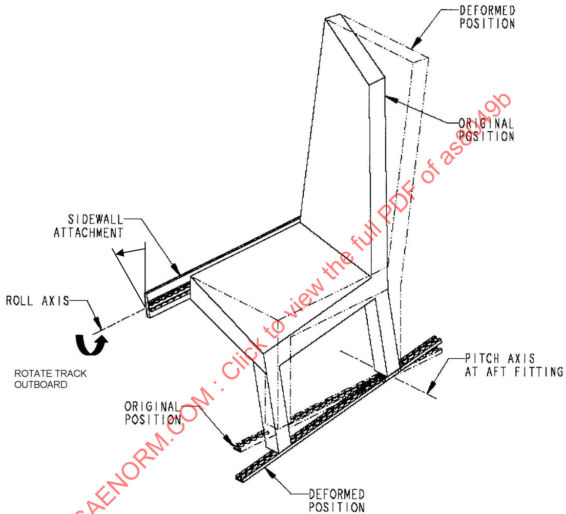
FIGURE 9D - Schematic of Floor Deformation: Side Wall Mounted Seat
