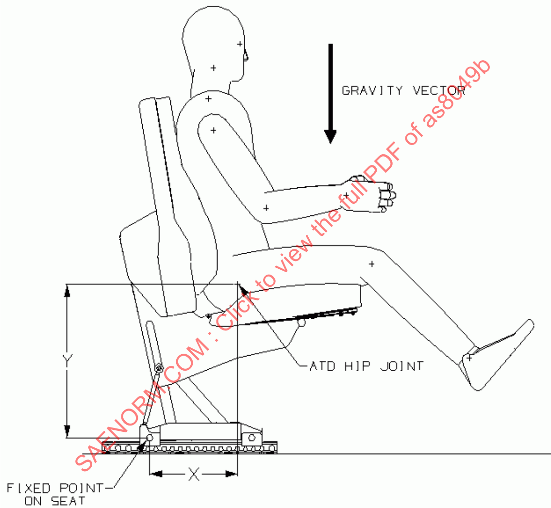
FIGURE 10 - Measurement of 1 g Preload
