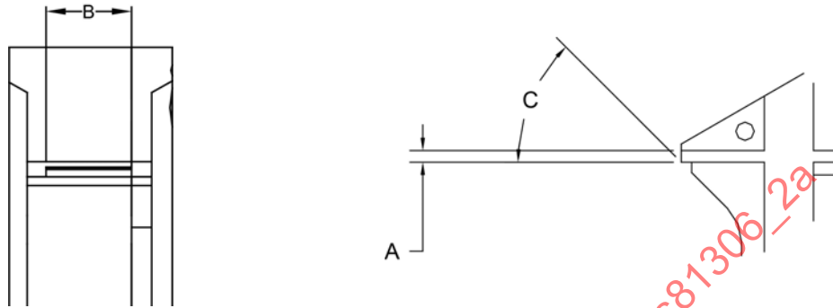
FIGURE 2 - NOSE DETAIL
