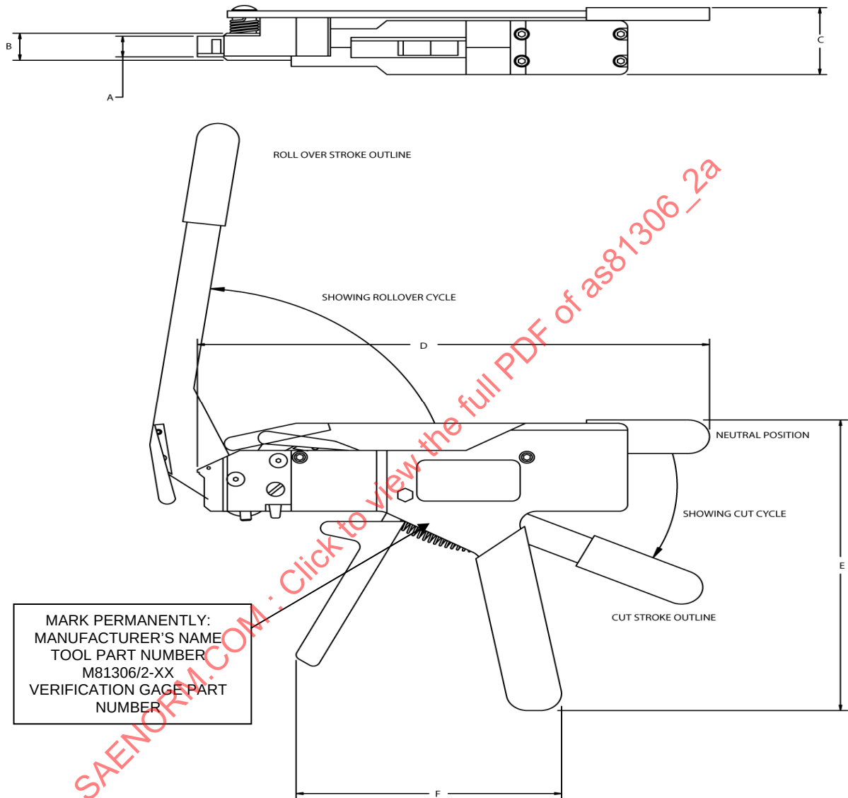
FIGURE 1 - DIMENSIONS AND CONFIGURATION
