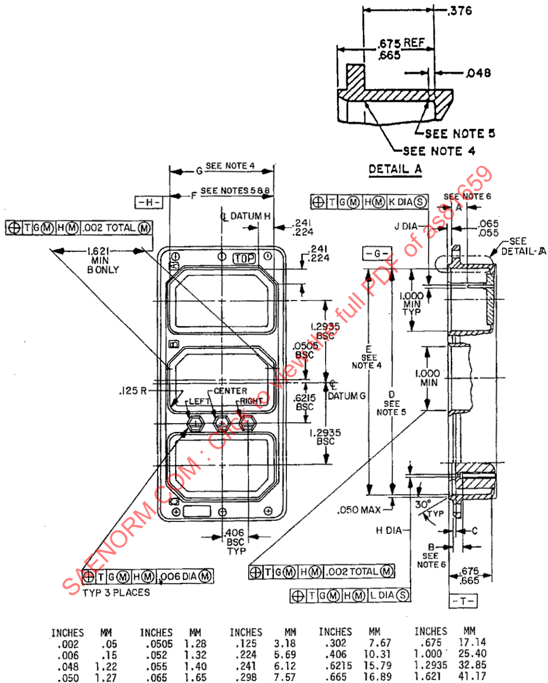
FIGURE 9. Triple receptacle connector intermateability control dimensions. (Shell designator A)
