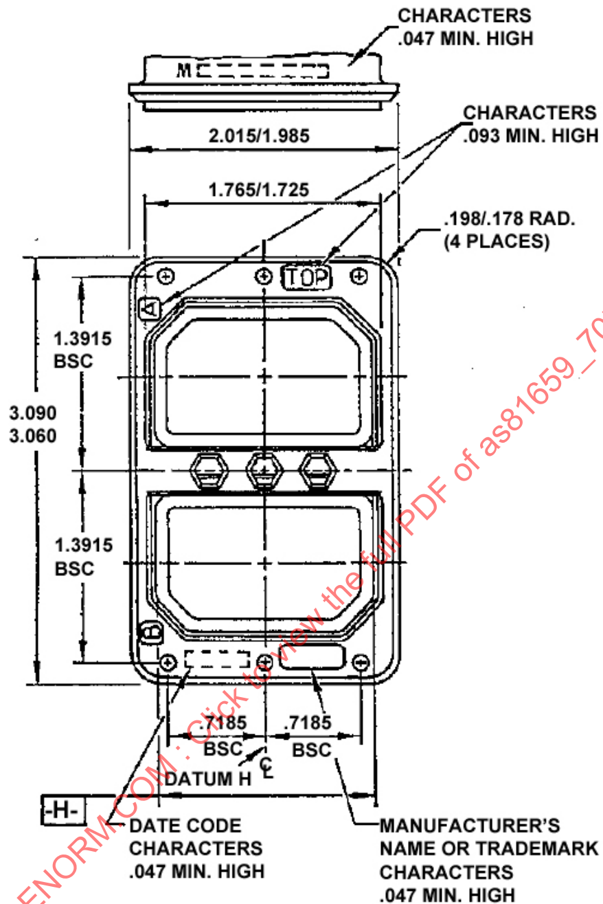
FIGURE 2 – CONNECTOR CONFIGURATIONS AND DIMENSIONS
