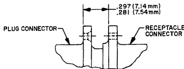
FIGURE 2 - DEFINITION OF A MATED CONNECTOR
