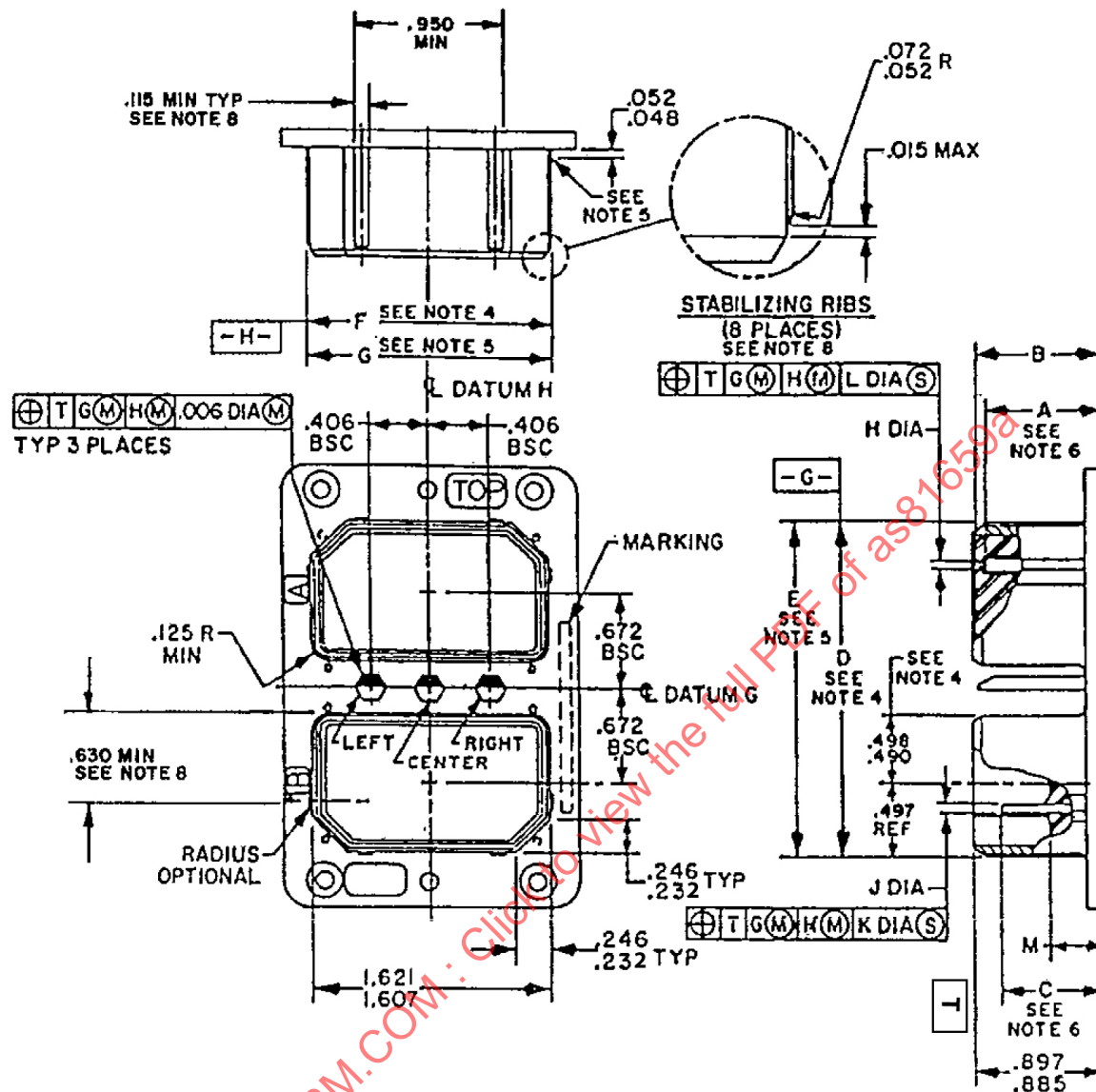
FIGURE 6 - DUAL PLUG CONNECTOR INTERMATEABILITY CONTROL DIMENSIONS (SHELL DESIGNATOR A)
