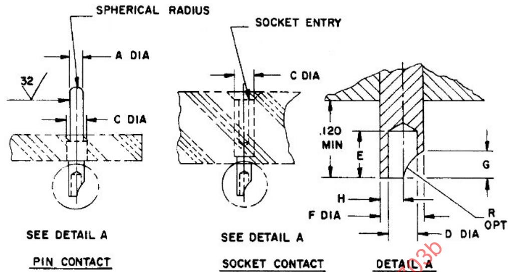
FIGURE 3 A. Contacts, solder type.
