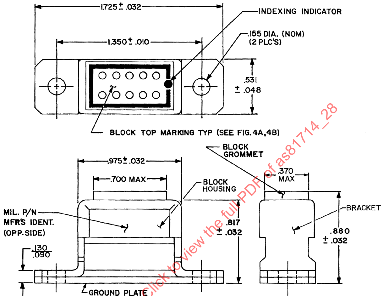
FIGURE 1. MOUNTING BRACKET HOUSING ONE BLOCK, SIZE 16.
