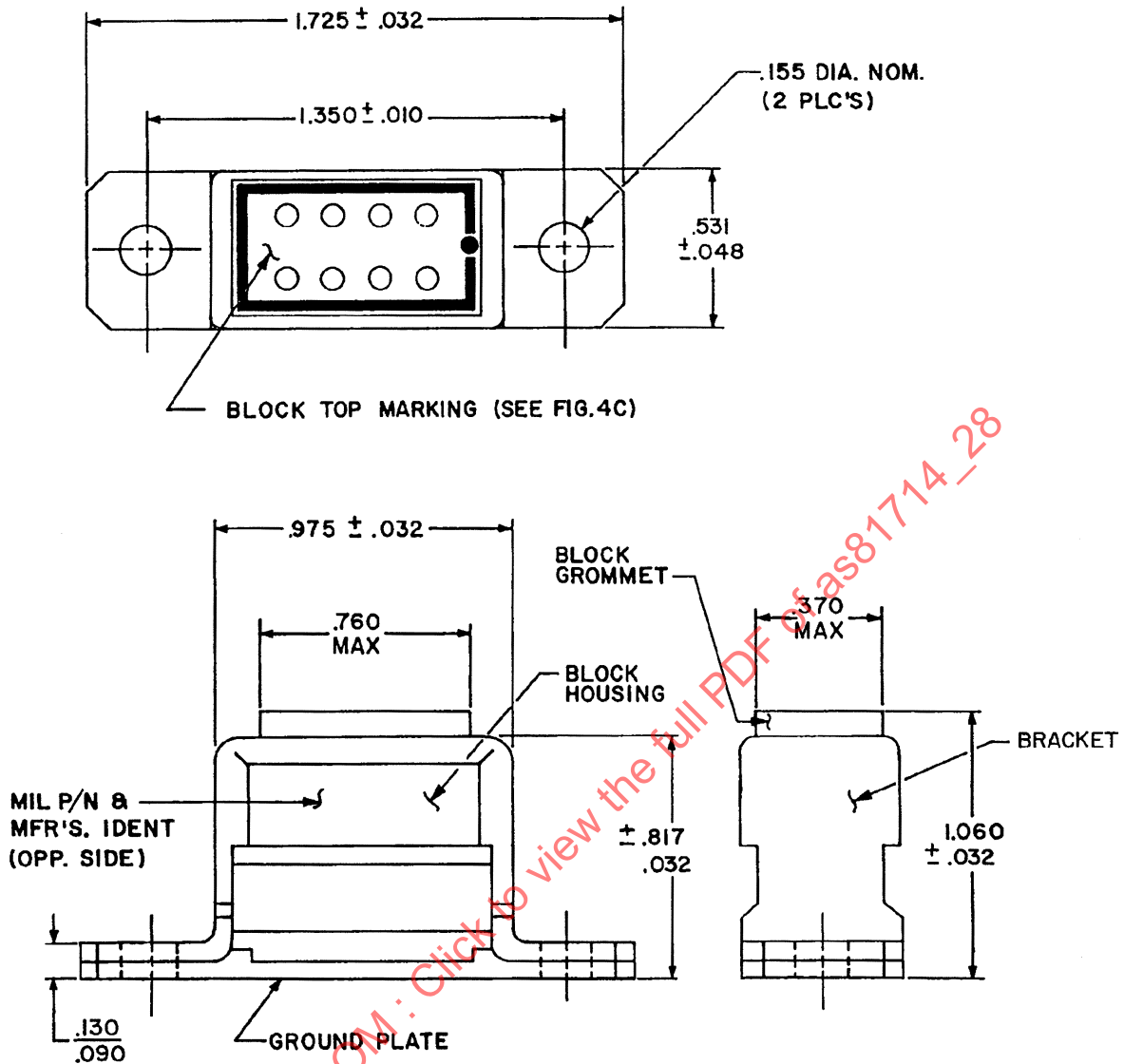
FIGURE 2. BRACKET MOUNTING GROUNDING BLOCK: SIZE 16.
