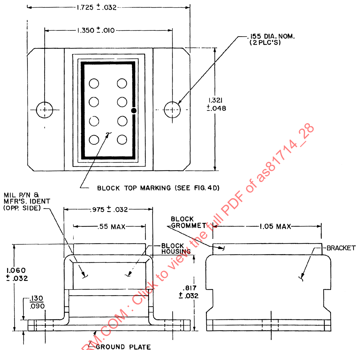
FIGURE 3. BRACKET MOUNTING GROUNDING BLOCK: SIZE 12.
