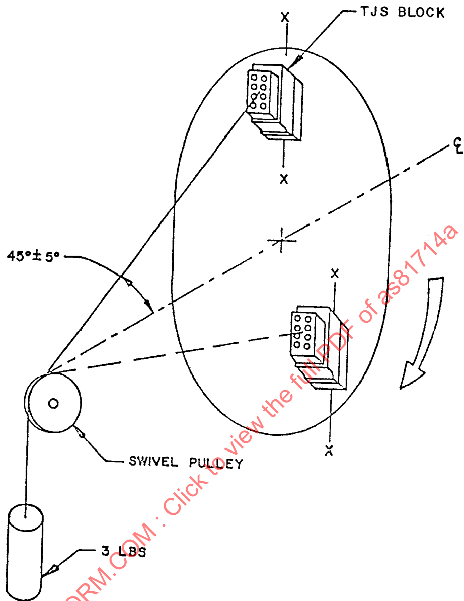
FIGURE 5 – CONTACT WALK-OUT TEST SETUP
