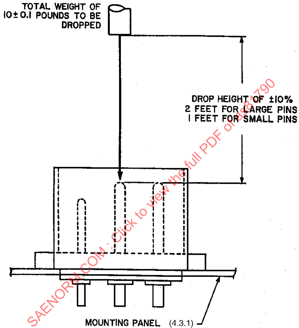
FIGURE 1. Method of performing pin impact strength test.
