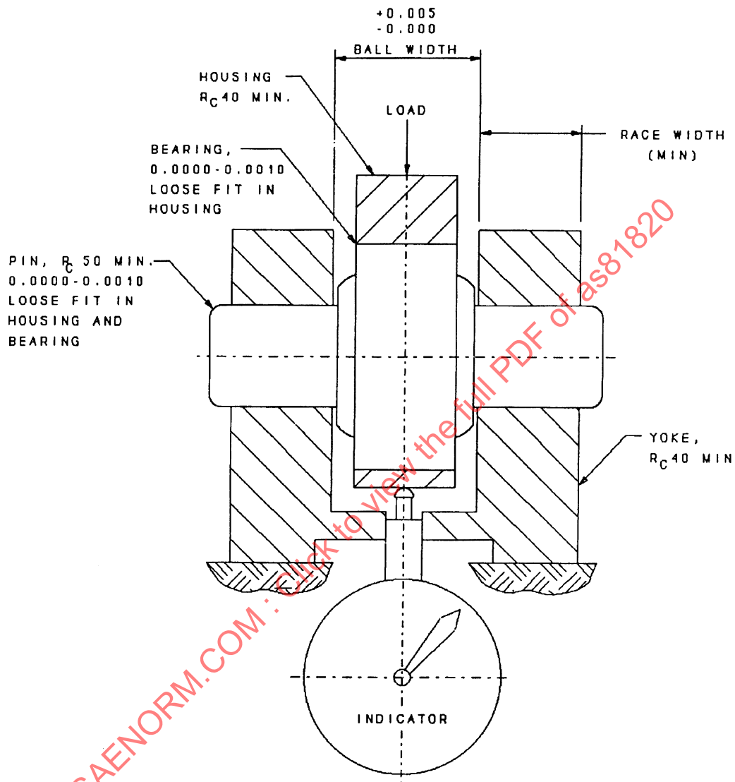
FIGURE 1. Radial static limit load test fixture.
