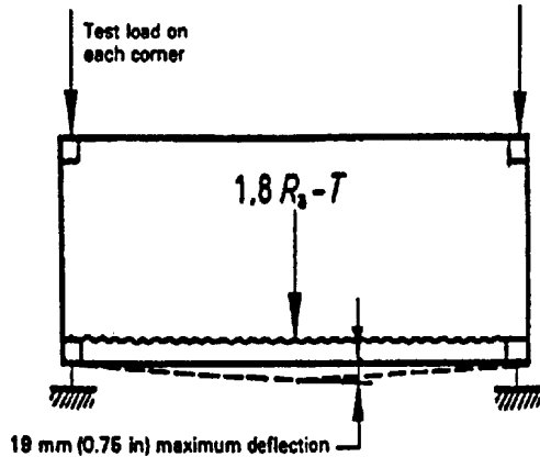
Test No. 1 - Stacking - Surface mode
