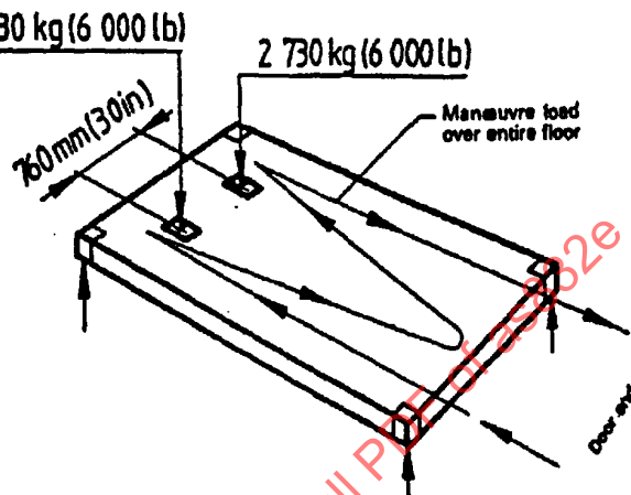
Test No 8.1 – Floor strength – Cyclic loading
