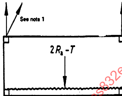
Test No. 2 - Top lifting - Surface mode
