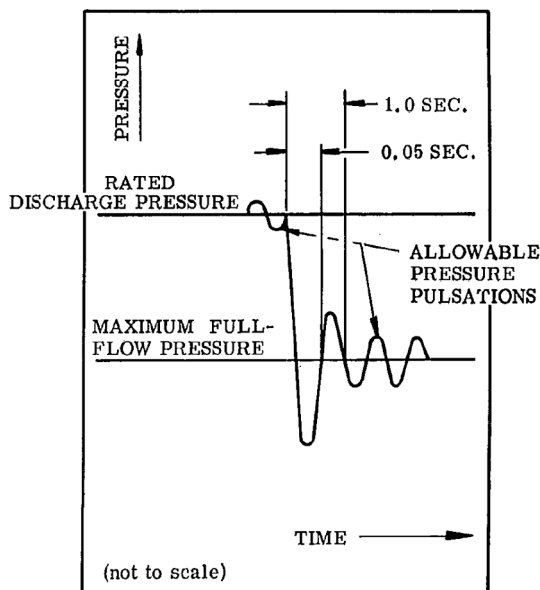
FIGURE 3. Typical pressure vs. time chart. For change from rated discharge pressure to maximum full-flow pressure (cutin).
