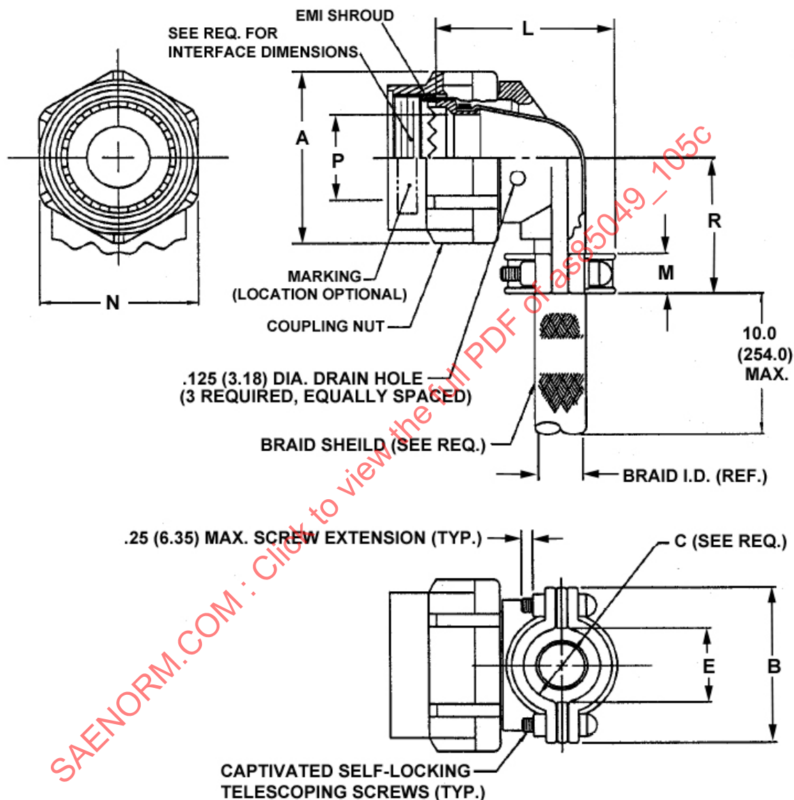
FIGURE 1 - ACCESSORY CONFIGURATION AND DIMENSIONS
