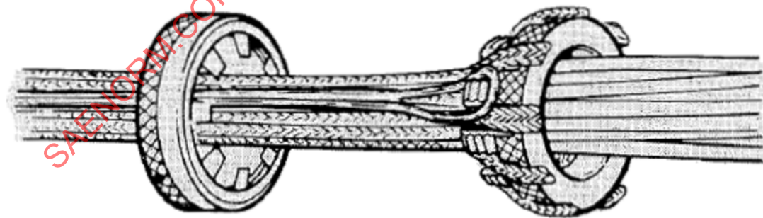
FIGURE 5 - STEP 4 OF ASSEMBLY INSTRUCTIONS
