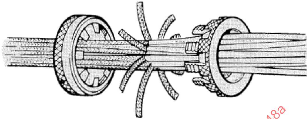
FIGURE 3 - STEP 2 OF ASSEMBLY INSTRUCTIONS
