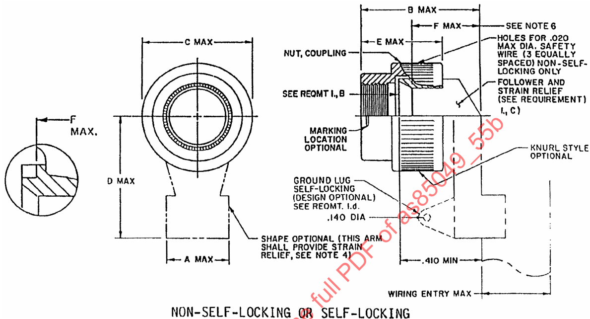
FIGURE 1 - CONFIGURATION AND DIMENSIONS
