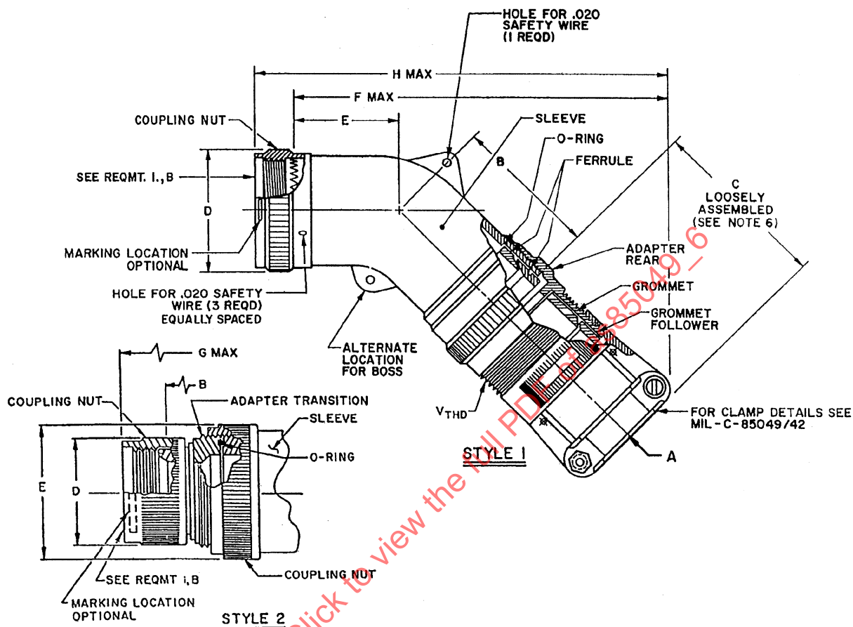
FIGURE 1. CONFIGURATION AND DIMENSIONS.
