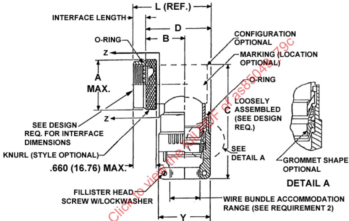
FIGURE 1 – ACCESSORY CONFIGURATION AND DIMENSIONS
