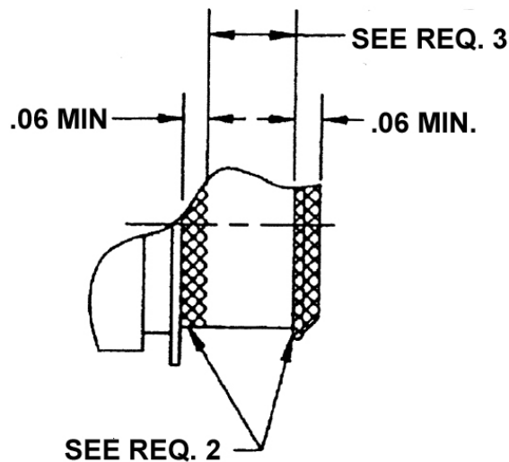
FIGURE 2 - SELECTIVE PLATING
