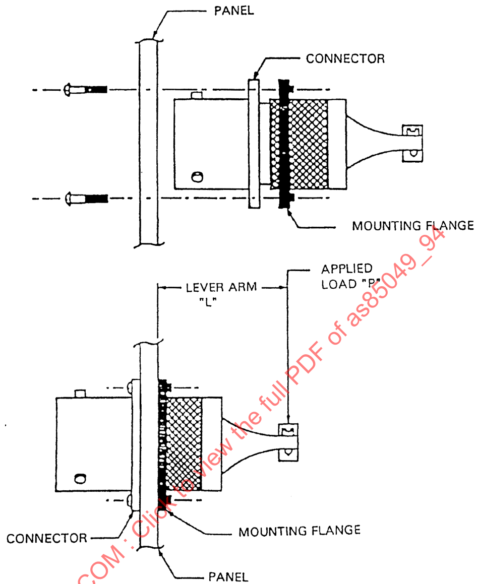
FIGURE 2. INSTALLATION - EXTERNAL BENDING MOMENT TEST SET-UP.
