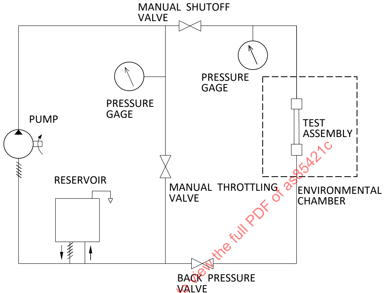
Figure 2 - Typical setup for thermal shock testing
