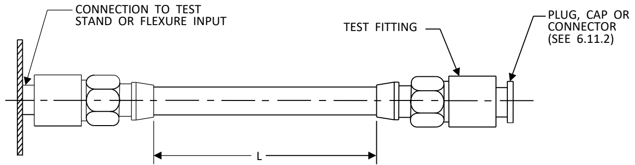
ASSEMBLY STYLE A
