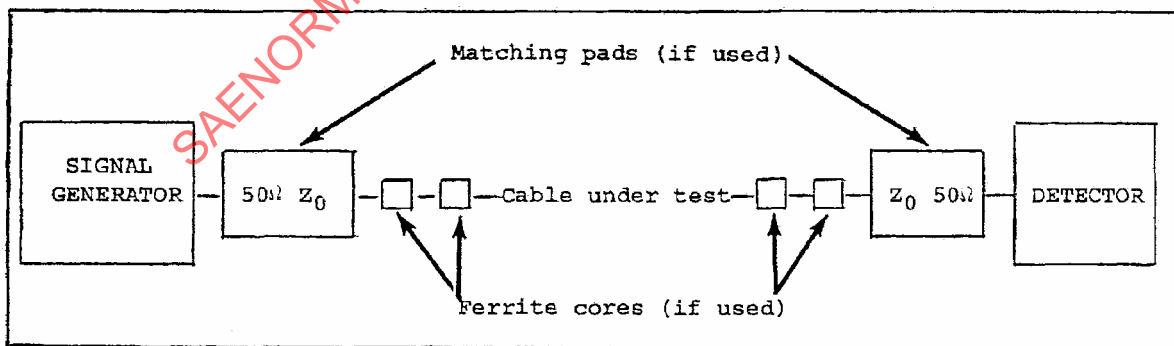
Figure 1. Configuration of specimen and test equipment.
