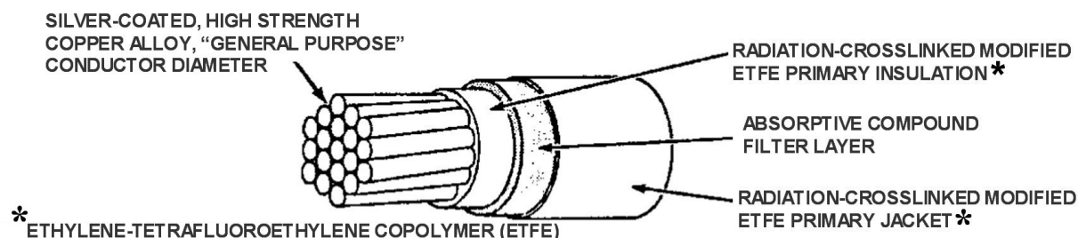
FIGURE 1 - AS85485/6 CONFIGURATION
