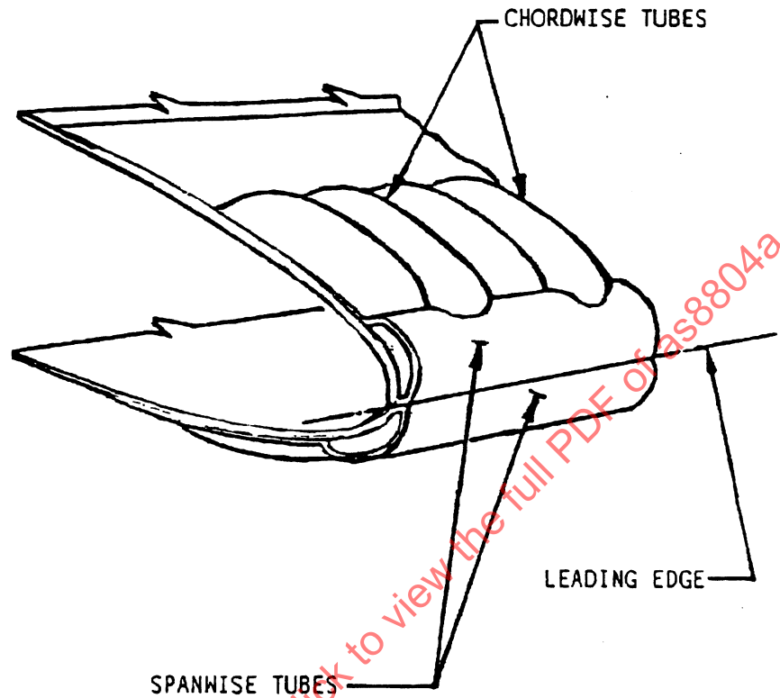
FIGURE 3. Rotorcraft blade pneumatic boot rotary wing aircraft.
