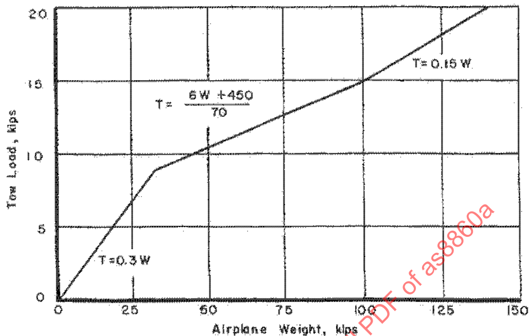
FIGURE 3 - Tow Loads (3.3.4.1 and 3.4.10.1)
