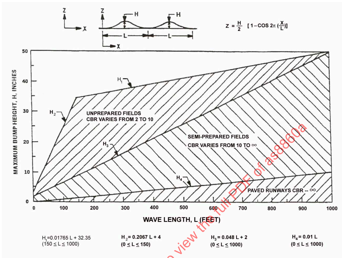
FIGURE 6 - Ground Roughness for Landing and Take-off (3.4.6)
