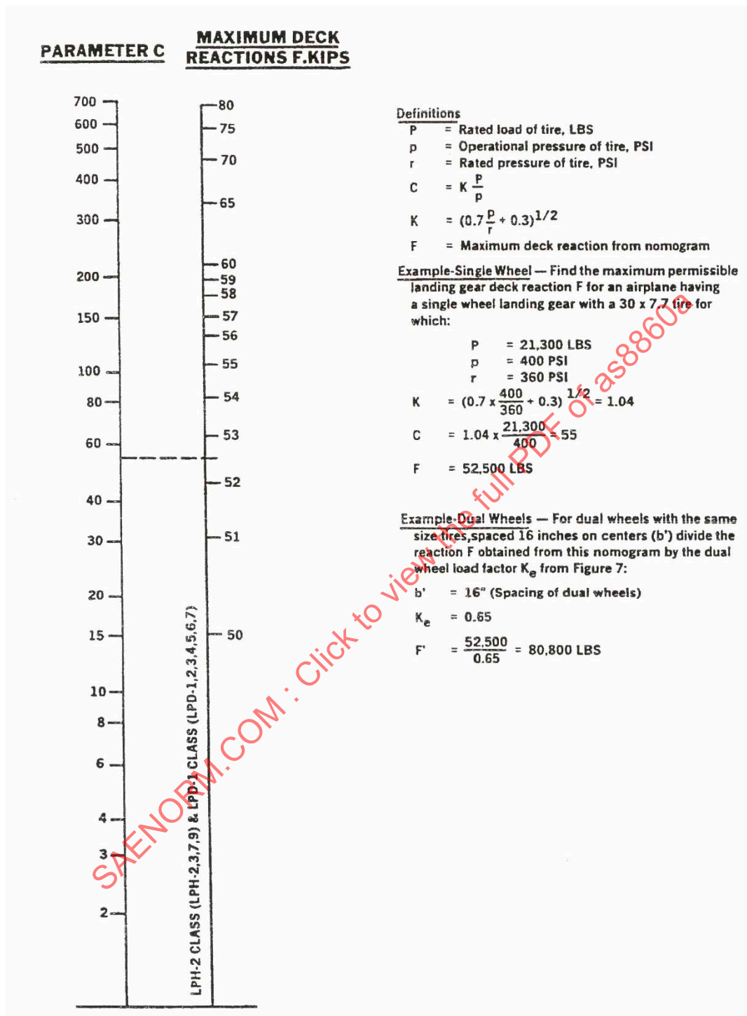
FIGURE 10 - Maximum Landing Reaction for Single Landing Gear With Single and Dual Wheels for Amphibious Warfare Ships (3.4.8.1.6)
