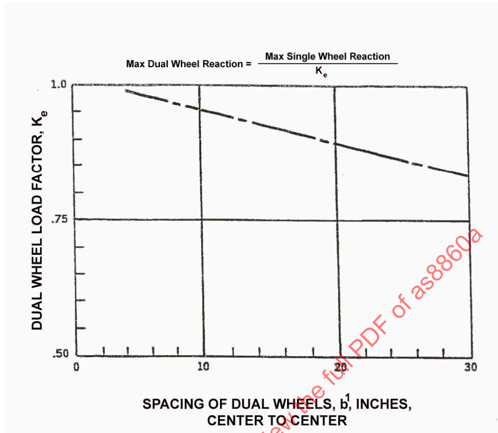
FIGURE 8 - Dual Wheel Load Factors (3.4.7.1.1)
