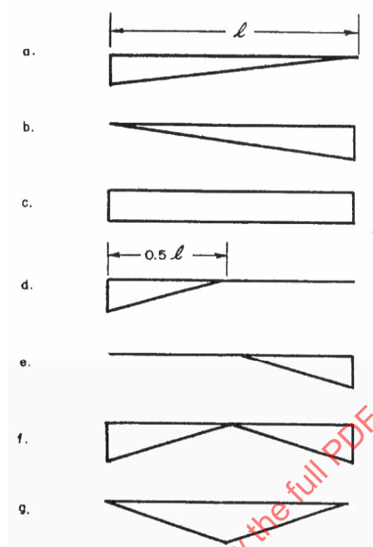
FIGURE 4 - Tire or Ski Load Distributions (3.3.6.3.1 and 3.4.11.4a,b)
