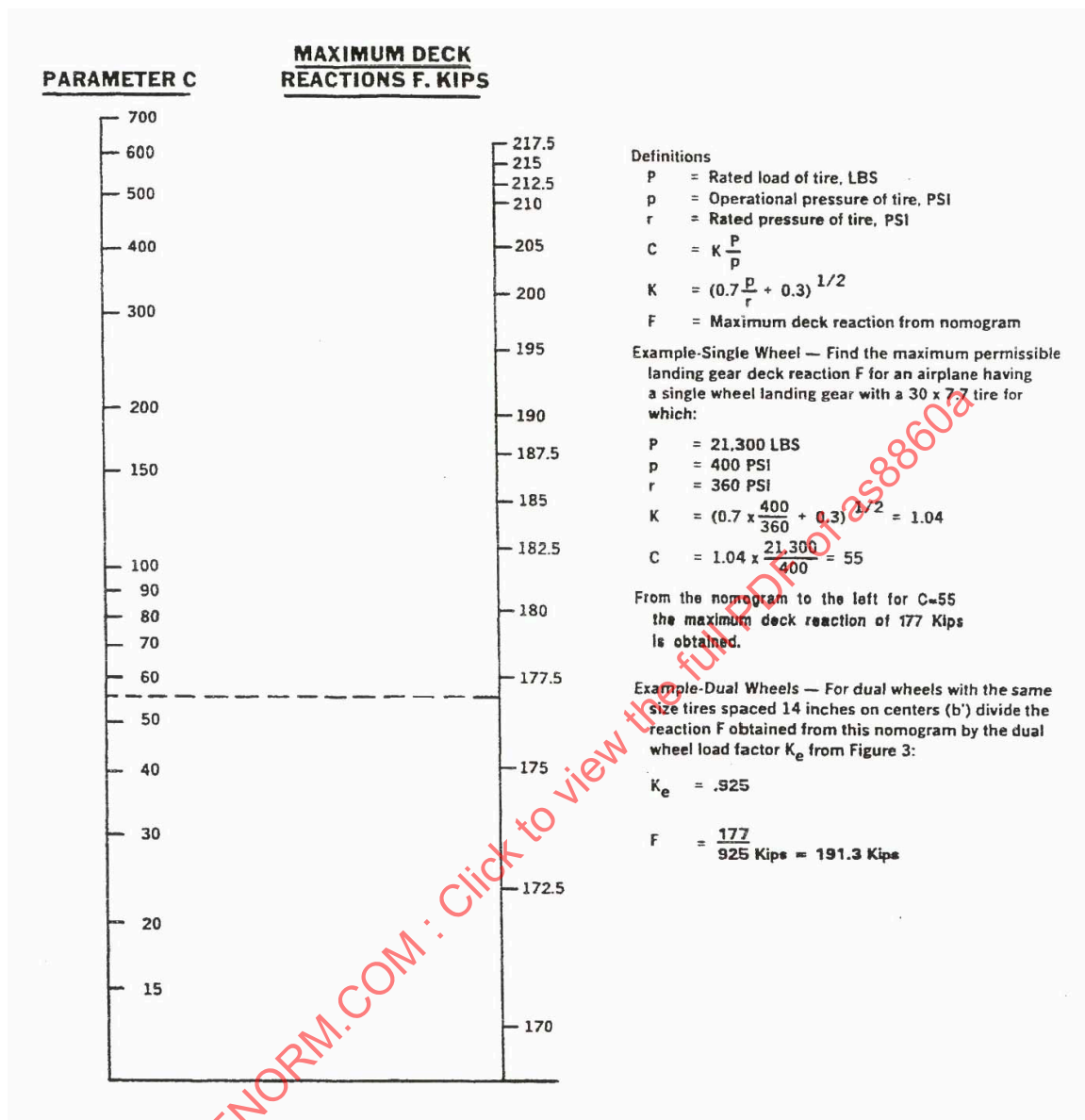
FIGURE 9—Maximum Allowable Vertical Deck Reaction for a Single Landing Gear - Landing Area on Aircraft Carriers (3.4.8.1.6)
