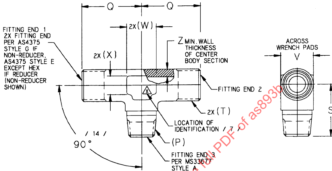
FIGURE 1 - FITTING, TEE, STANDARD AND REDUCER, FLARELESS TUBE TO PIPE ON SIDE, EXTERNAL THREAD
