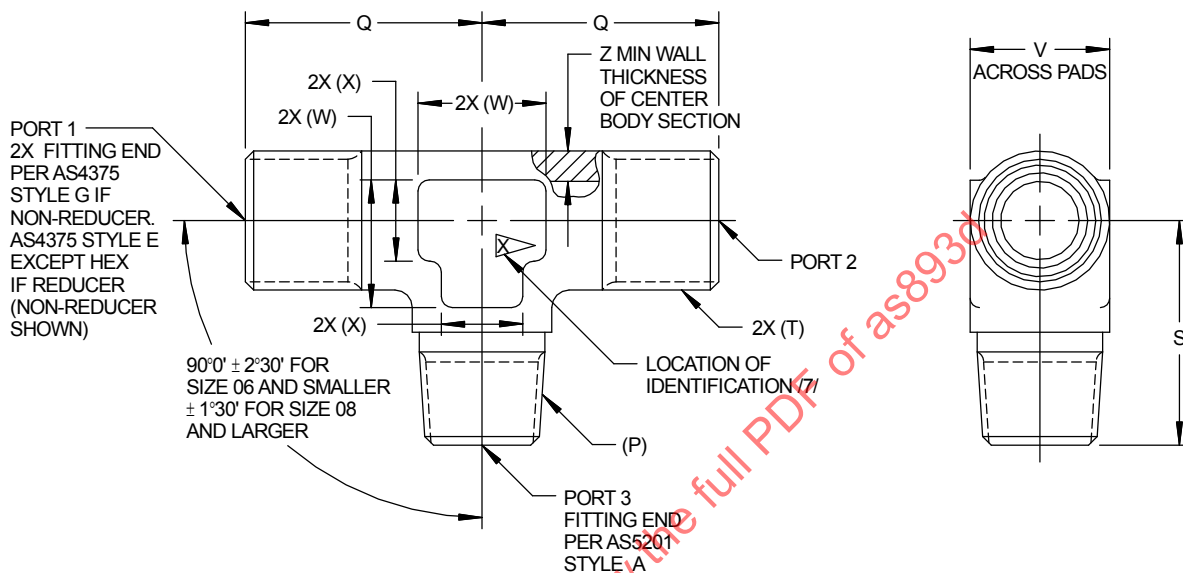
FIGURE 1 – FITTING, TEE, STANDARD AND REDUCER, FLARELESS TUBE TO PIPE ON SIDE, EXTERNAL THREAD
