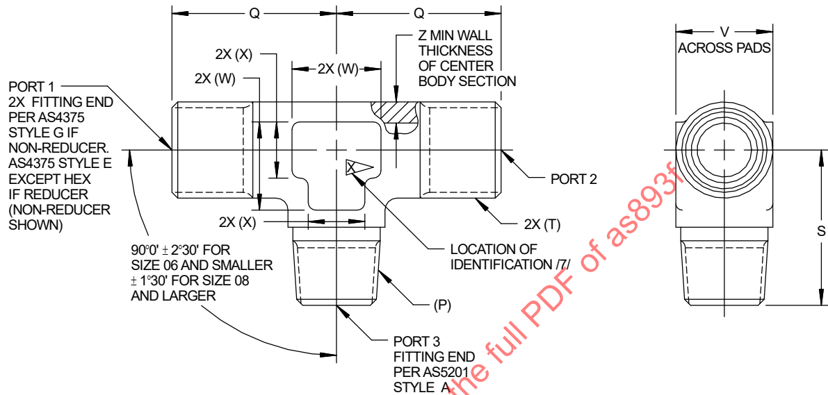
FIGURE 1 - FITTING, TEE, STANDARD AND REDUCER, FLARELESS TUBE TO PIPE ON SIDE, EXTERNAL THREAD
