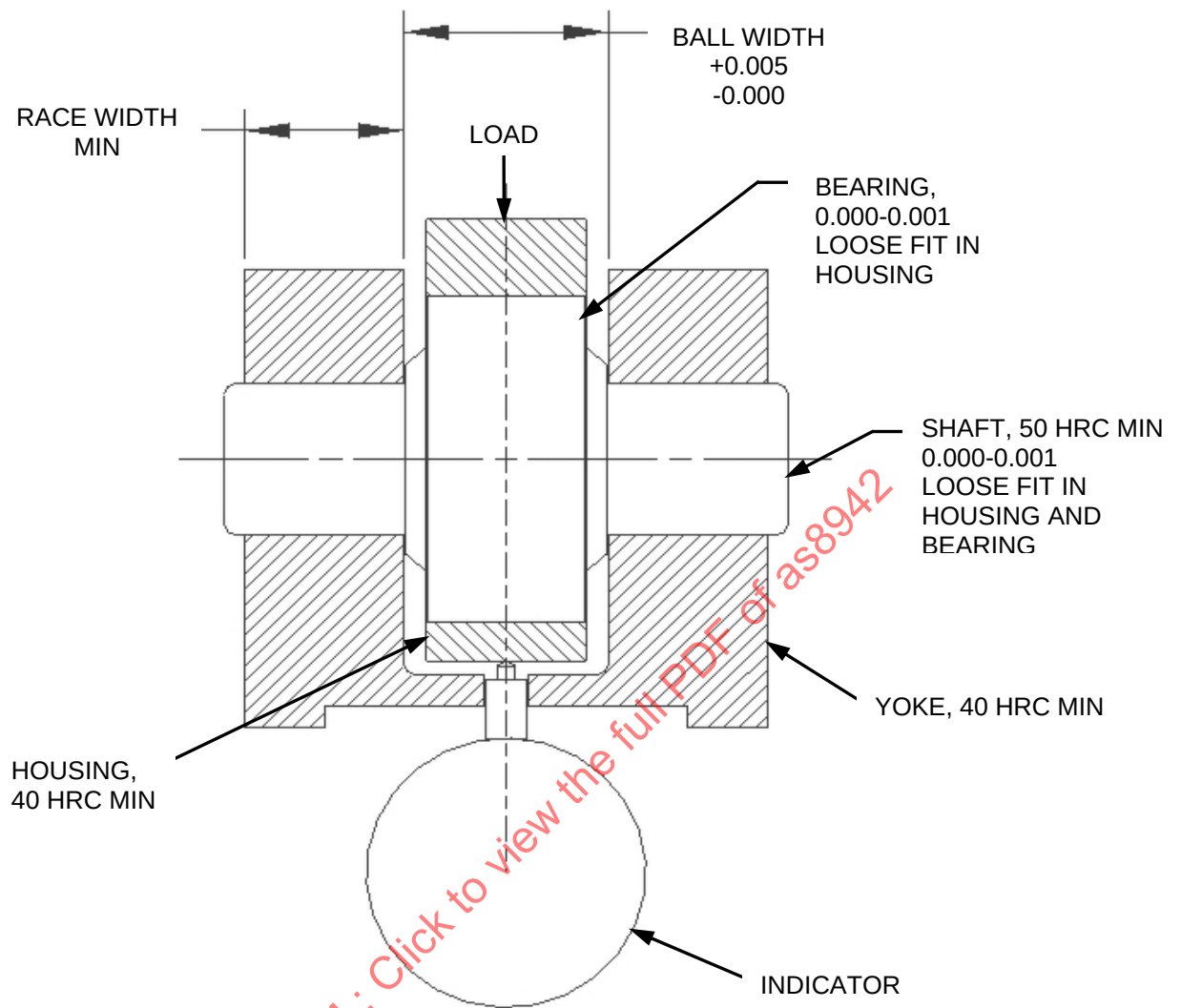
FIGURE 1 – RADIAL TEST FIXTURE
