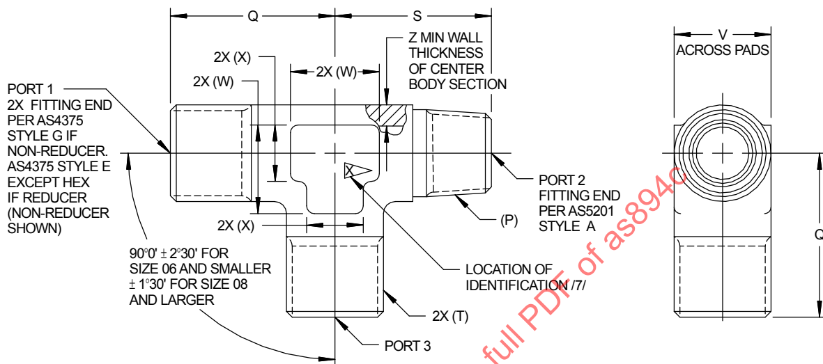
FIGURE 1 - FITTING, TEE, STANDARD AND REDUCER, FLARELESS TUBE TO PIPE ON RUN, EXTERNAL THREAD
