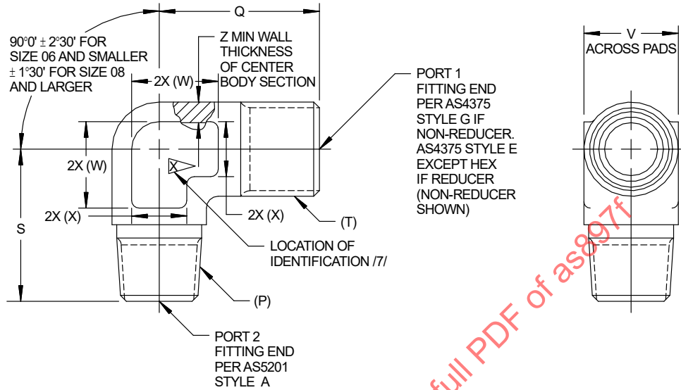
FIGURE 1 - FITTING, ELBOW, 90°, STANDARD AND REDUCER, FLARELESS TUBE TO PIPE, EXTERNAL THREAD
