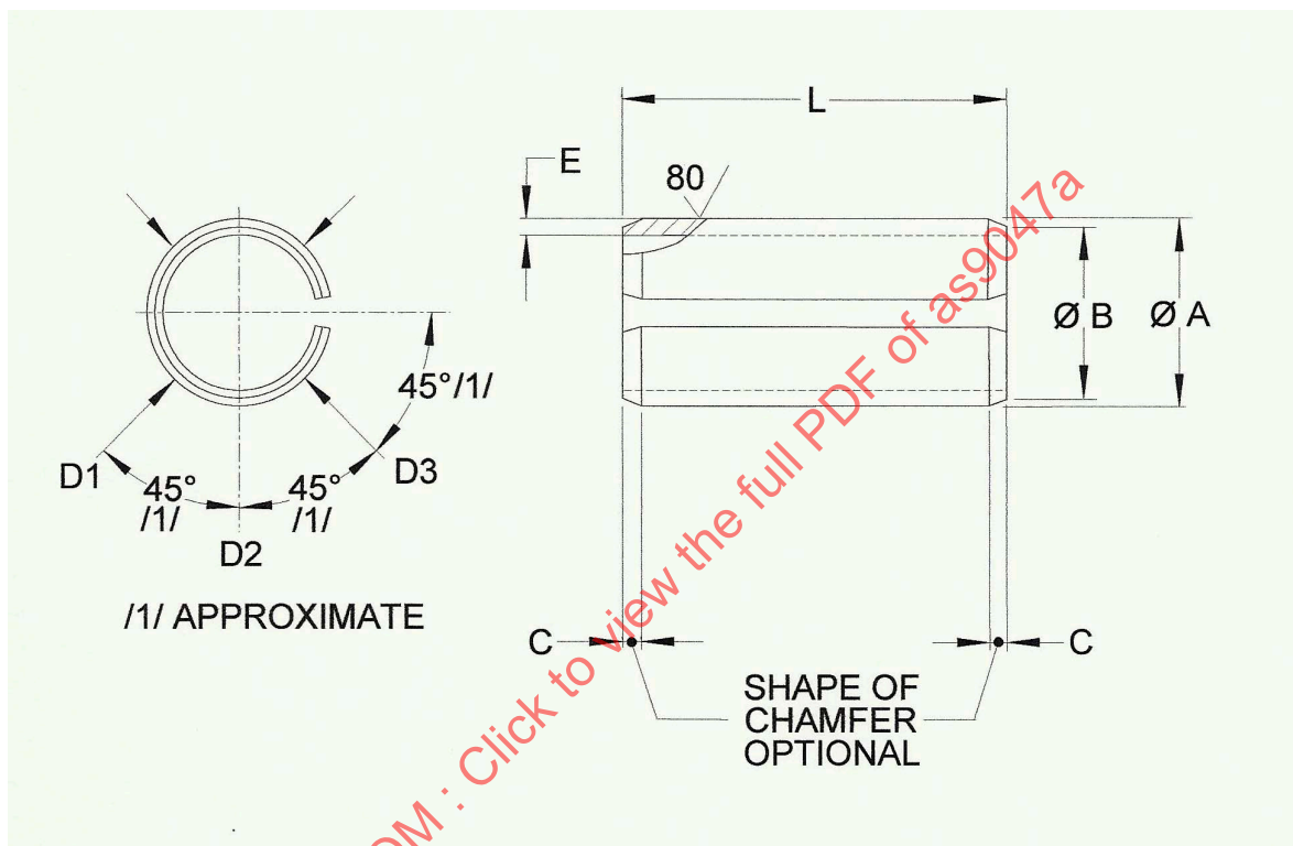
FIGURE 1 - PIN
