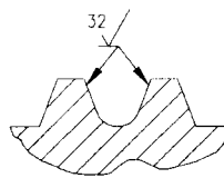
SECTION THRU THREAD PROFILE
