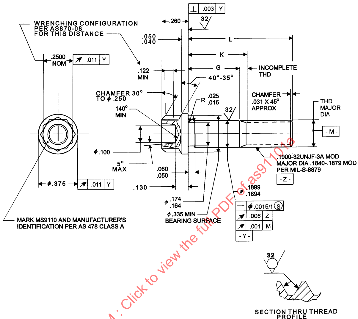
FIGURE 1 - BOLT
