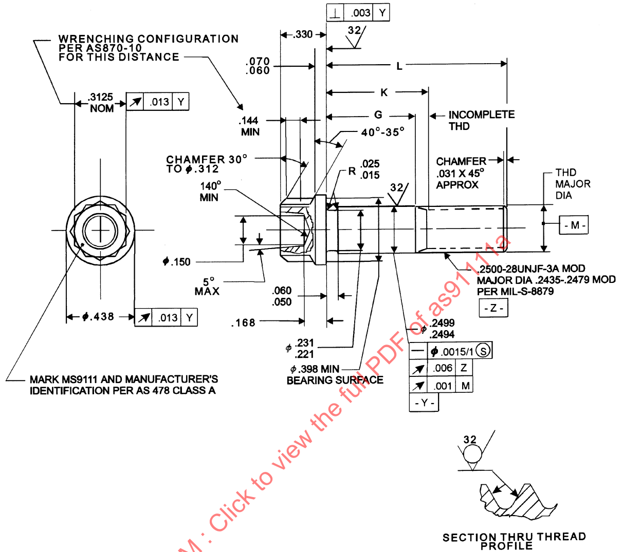
FIGURE 1 - BOLT
