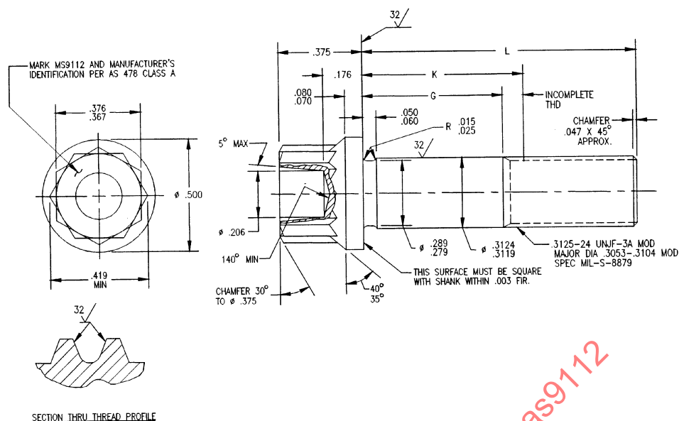
FIGURE 1 - BOLT
