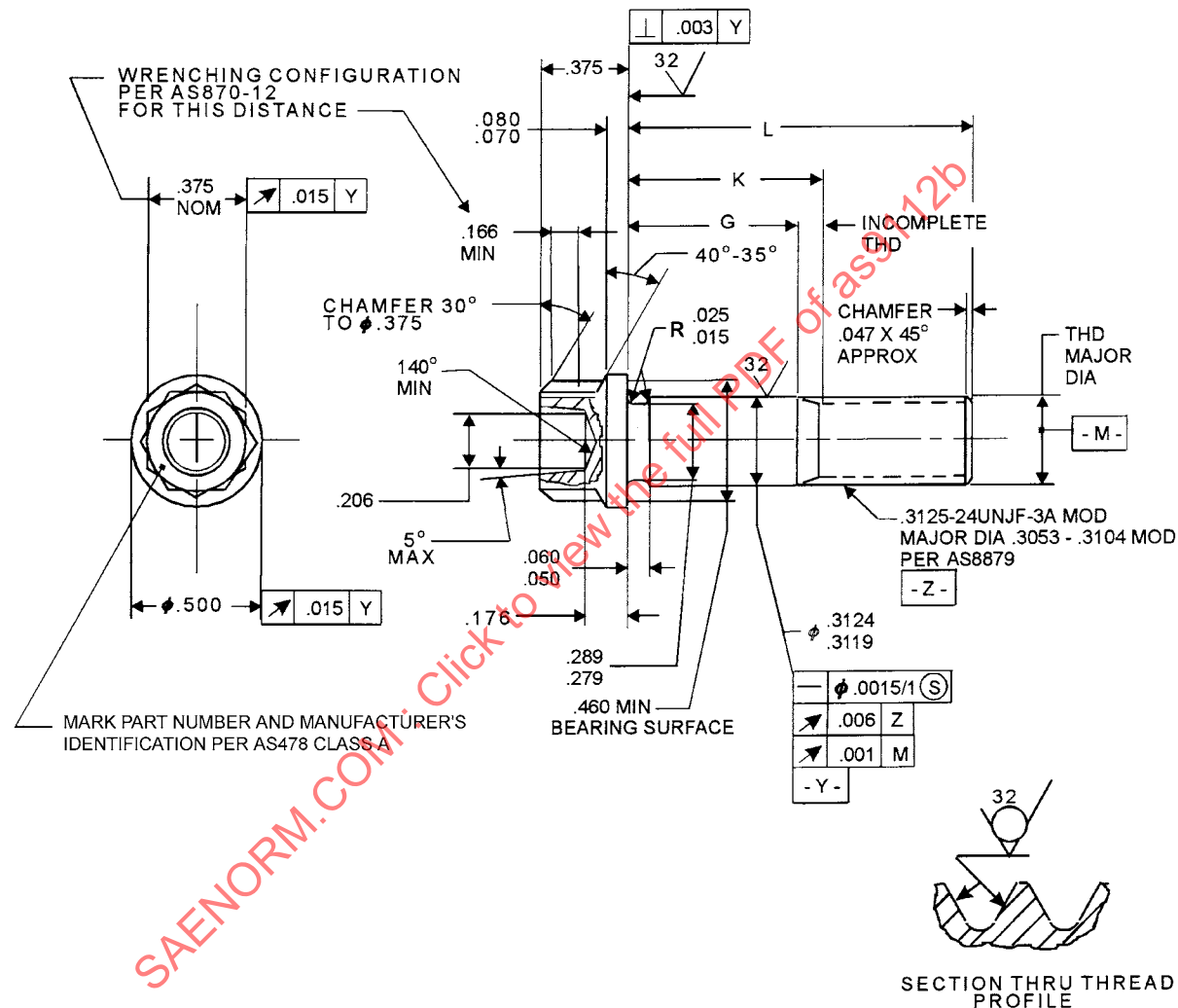
FIGURE 1 - BOLT
