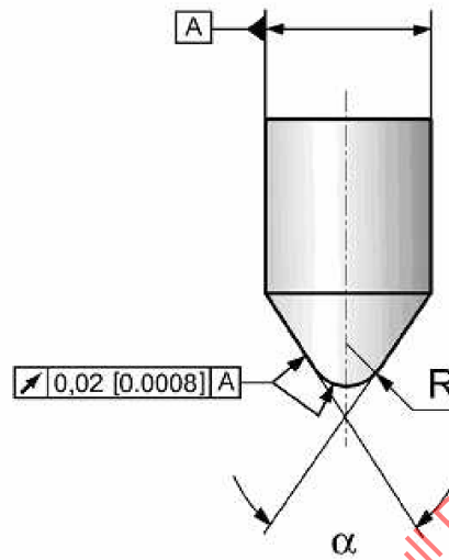
FIGURE B1 - Tolerance on Stylus
