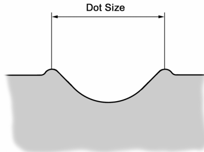
FIGURE 7 - Detail Definition of Dot Size
