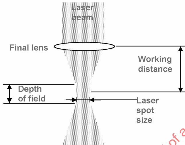
FIGURE 9 - Diagram Illustrating Typical Laser Beam Profile at Working Range
