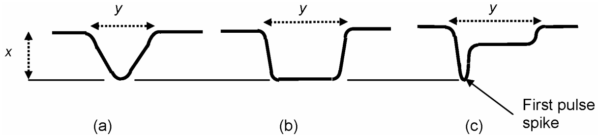
FIGURE 13 - Diagram Showing Different Laser Engraved Module Profiles, All of These Will Have the Same Module Depth (x)
