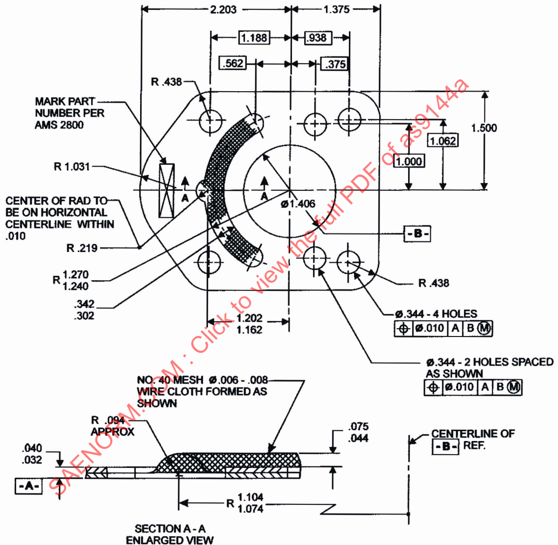
FIGURE 1 - GASKET
