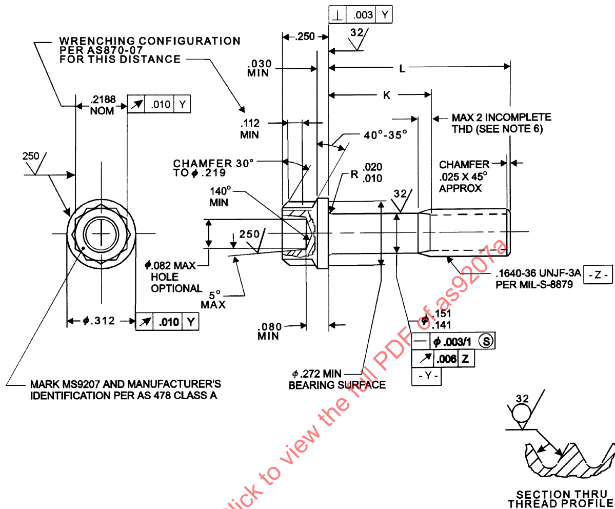
FIGURE 1 - SCREW
