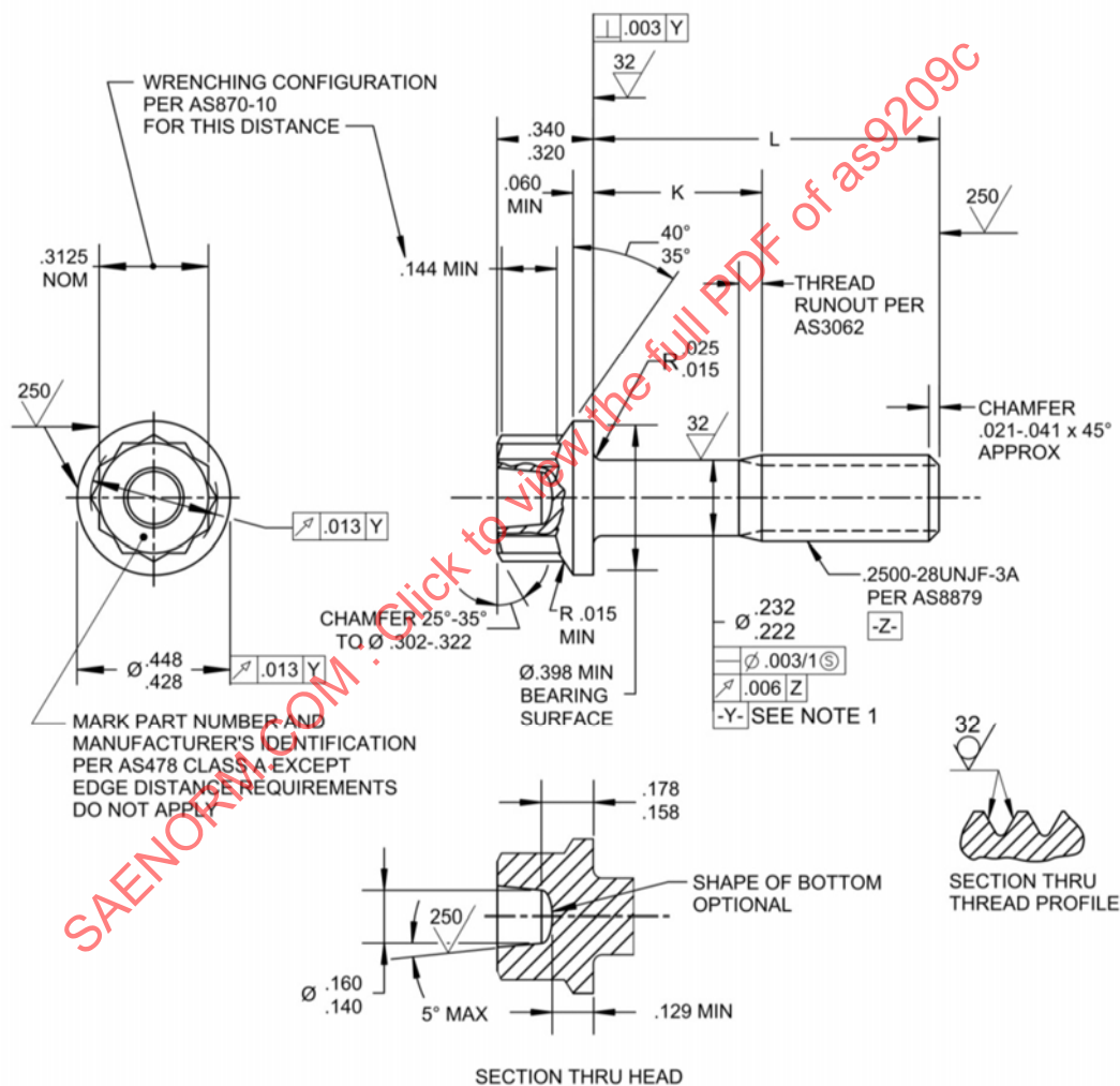
FIGURE 1 - BOLT
