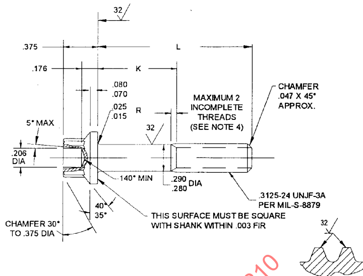
SECTION THROUGH THREAD PROFILE
