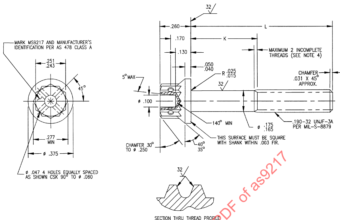
FIGURE 1 - BOLT
