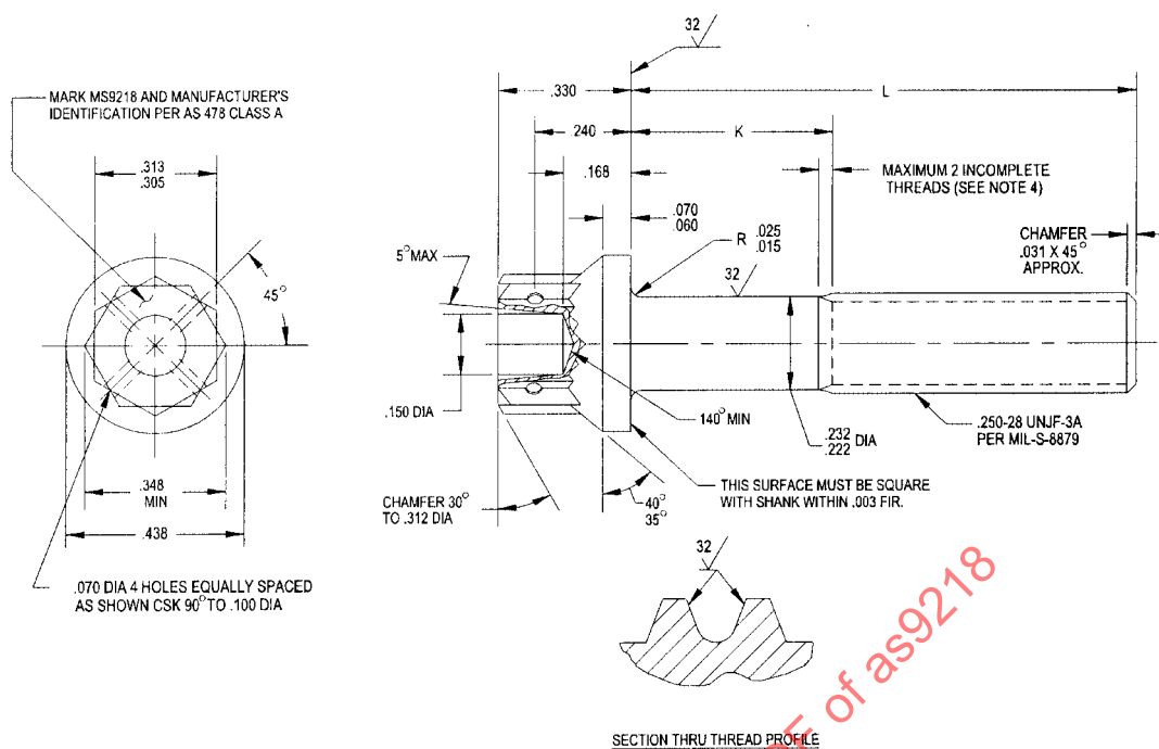
FIGURE 1 - BOLT
