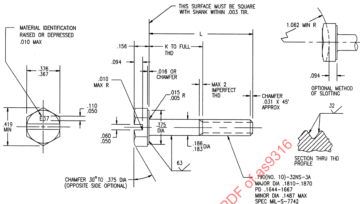
FIGURE 1 - SCREW
