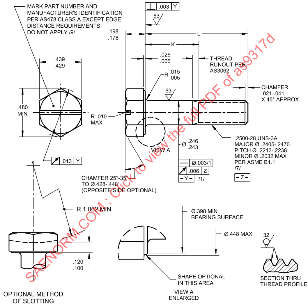
FIGURE 1 - SCREW
