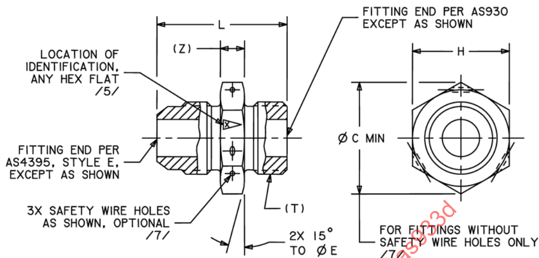
FIGURE 1 – FITTING, ADAPTER, UNION
