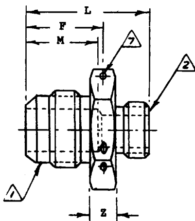
REDUCER ADAPTER
