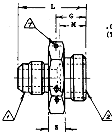
EXPANDER ADAPTER
